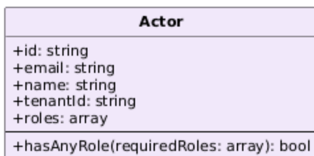
Figura 81: Classe: Actor
