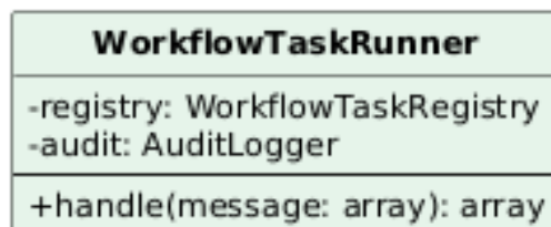
Figura 76: Classe: WorkflowTaskRunner
