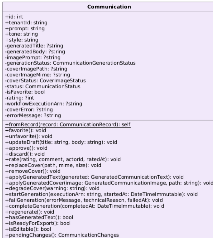
Figura 53: Classe: Communication
