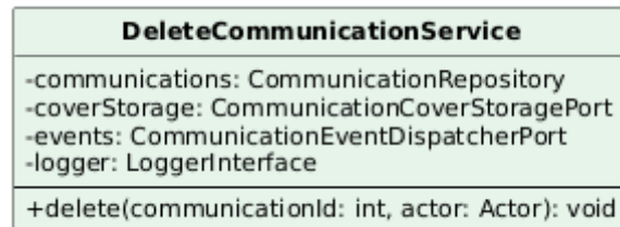
Figura 66: Classe: DeleteCommunicationService
