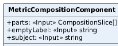
Figura 118: Classe: MetricCompositionComponent
